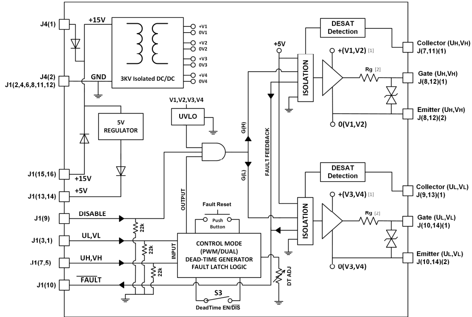
Figure 1: Block Diagram
